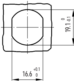
Drilling template
