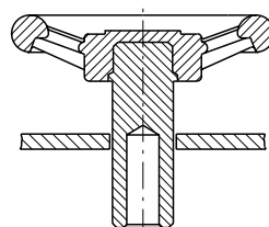
Extended boss for bulkhead assembly
