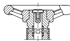
Extended boss and claw coupling
