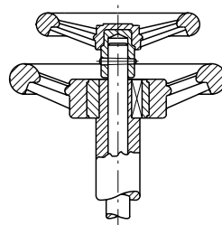
Controlling coaxial shafts
