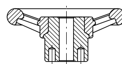
Extended boss and spring-loaded ball locking mechanism
